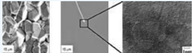
Conventional nickel deposit (left) and nanocrystalline deposit (center and right).
